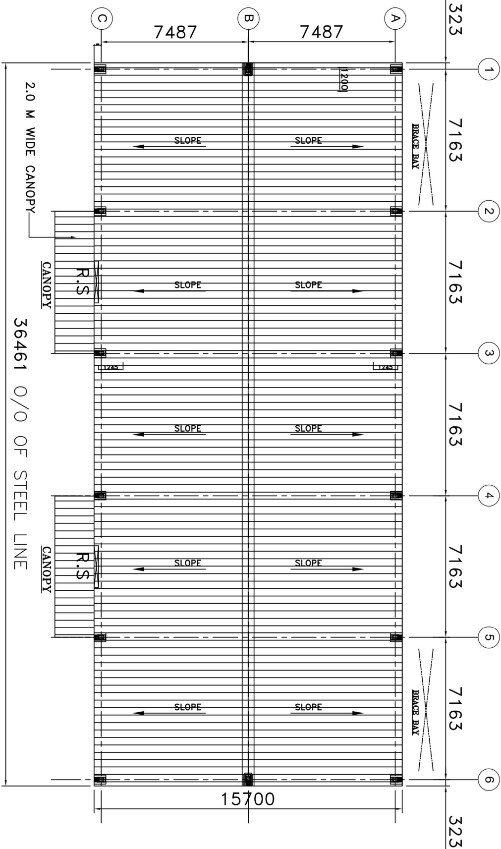
ROOF LAYOUT PLAN
